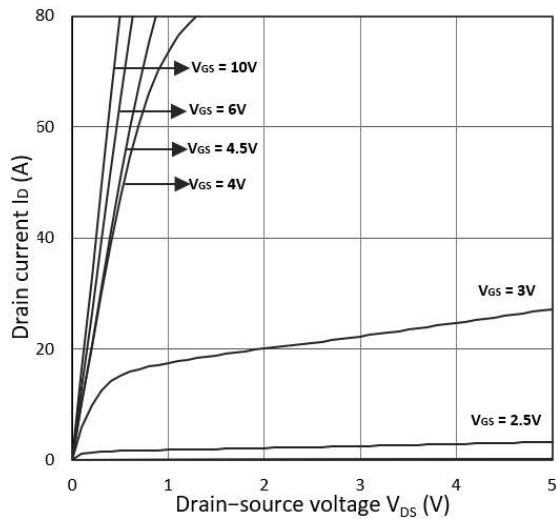
Figure 1. Output Characteristics
