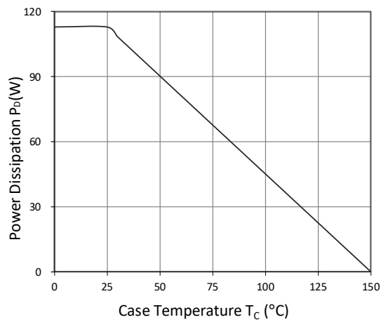
Figure 9. Power Dissipation
