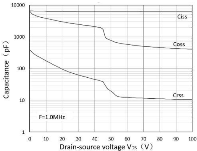
Figure 7. Capacitance Characteristics
