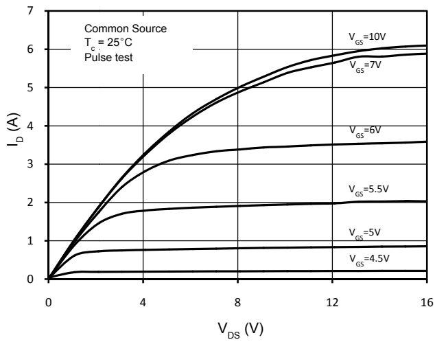
Figure 1. On-Region Characteristics
