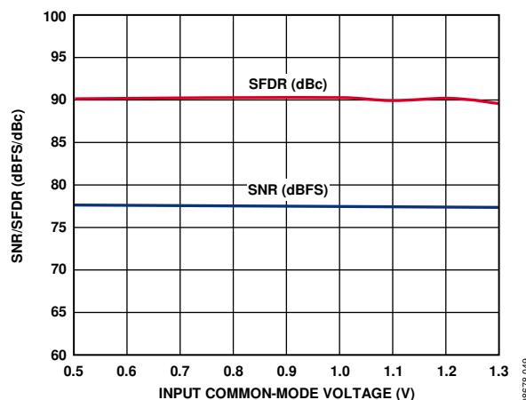
Figure 36. SNR/SFDR vs. Input Common-Mode Voltage, f_{IN} = 32.5 \text{ MHz} , f_s = 80 \text{ MSPS}
