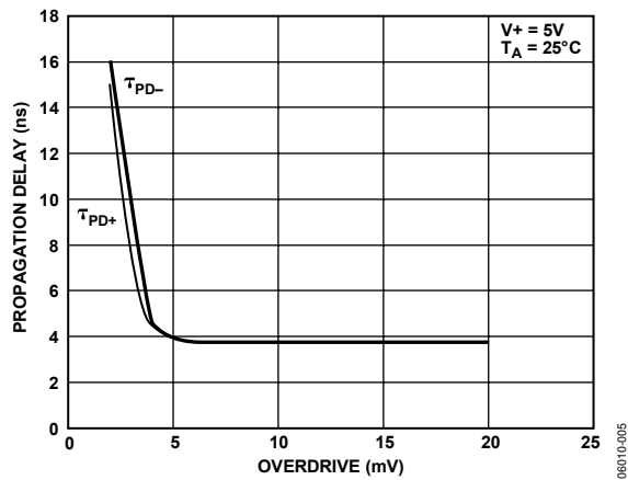
Figure 8. Propagation Delay vs. Overdrive
