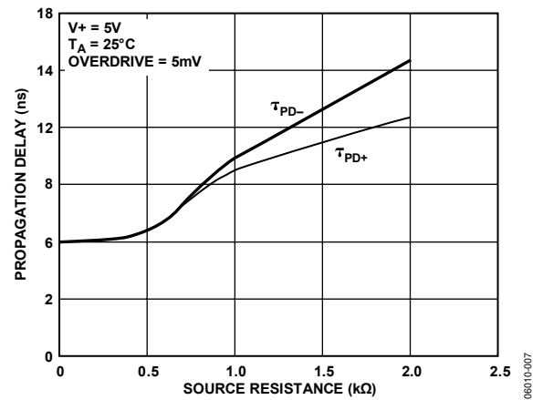
Figure 10. Propagation Delay vs. Source Resistance
