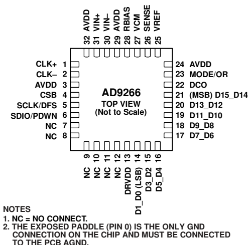
Figure 3. Pin Configuration
