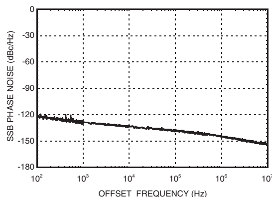
SSB Phase Noise Performance, Fout= 16 GHz, Input Power = +3 dBm
