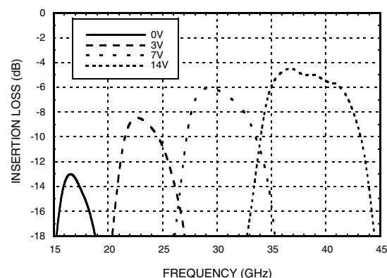
Insertion Loss vs. V_{ctl}
