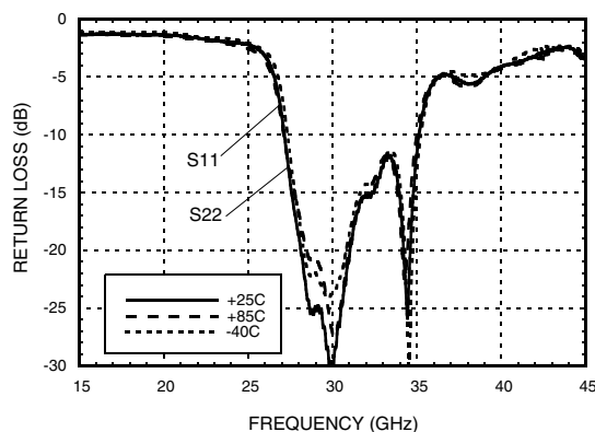
Return Loss vs. Temperature, V_{ctl} = 7V
