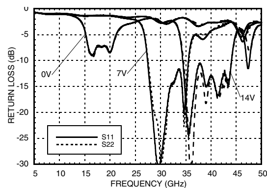
Broadband Return Loss vs. V_{ctl}
