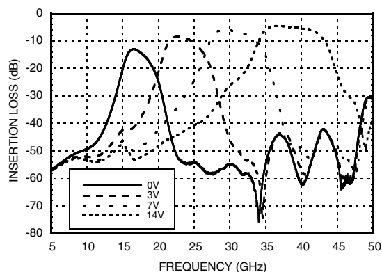
Broadband Insertion Loss vs. V_{ctl}
