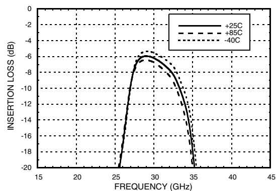
Insertion Loss vs. Temperature, V_{ctl} = 7V
