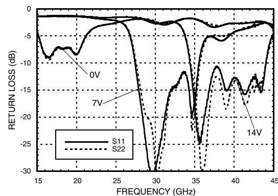
Return Loss vs. V_{ctl}
