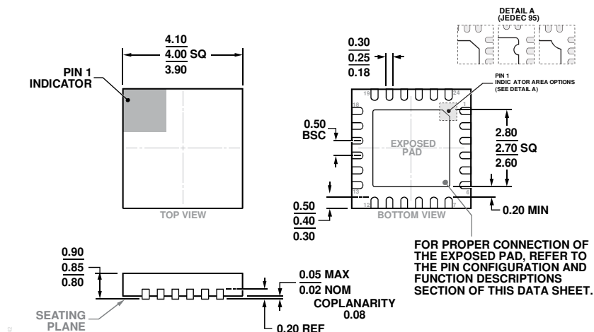
Figure 23. 24-Lead Lead Frame Chip Scale Package [LFCSP] 4 mm x 4 mm Body and 0.85 mm Package Height (CP-24-16) Dimensions shown in millimeters
