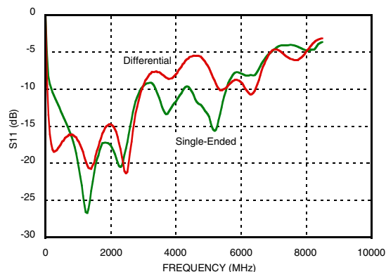
Figure 20. S-Parameters - S11 [11]
