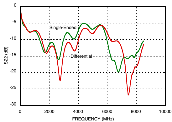
Figure 22. S-Parameters - S22 [11]
