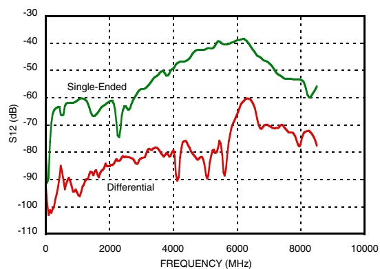
Figure 21. S-Parameters - S12 [11]
