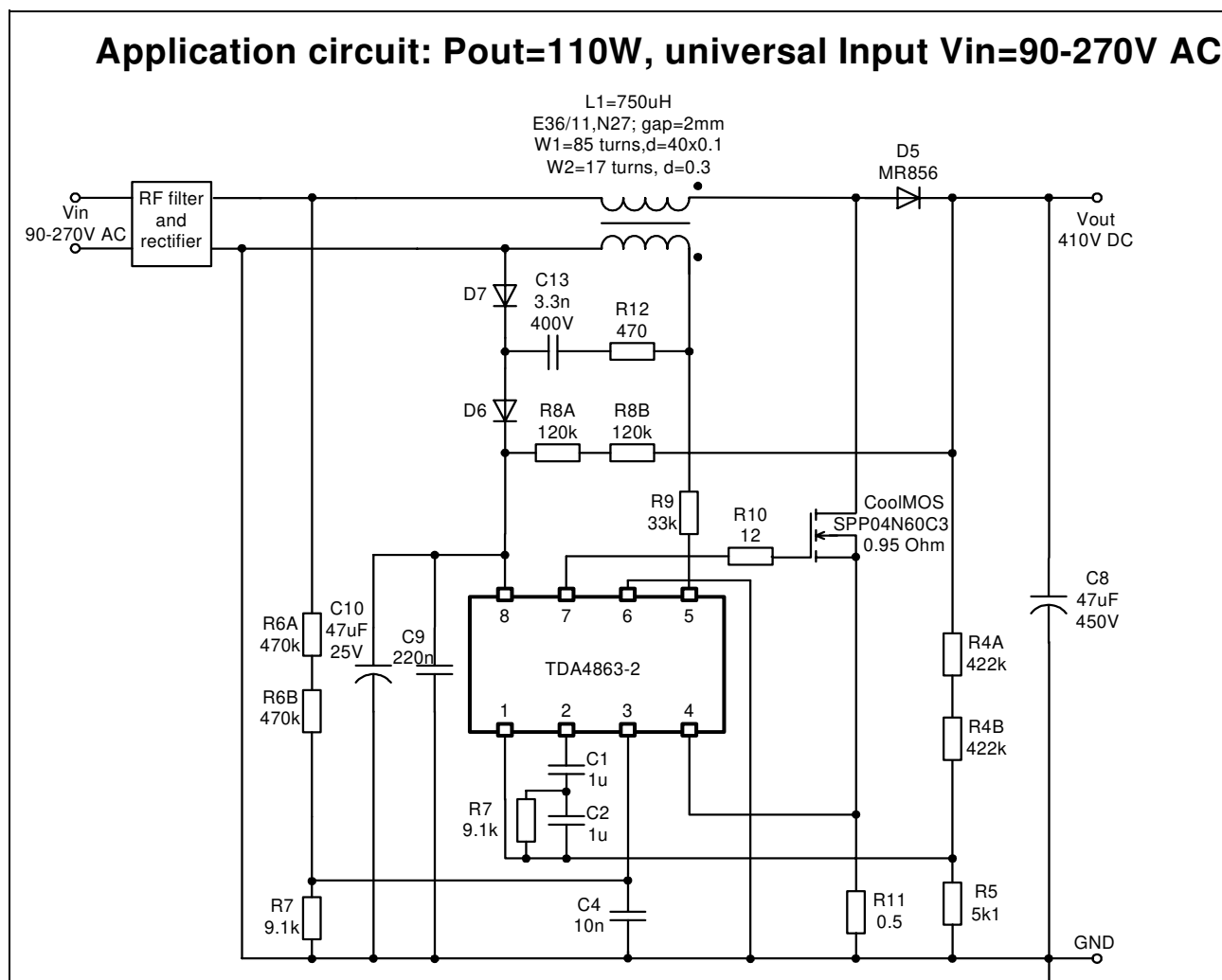
Figure 5 P_{out} = 110 \text{ W} , Universal Input V_{in} = 90 - 270 \text{ V AC}
